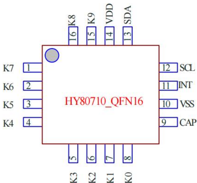
QFN16(3*3mm)
